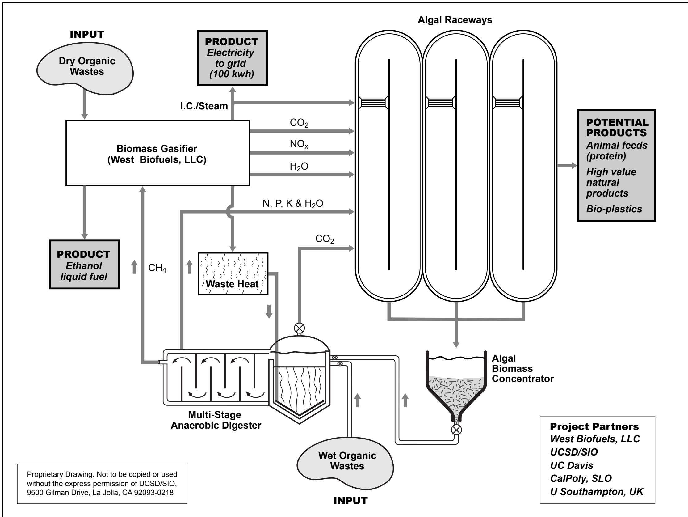
Proposed Woodland, CA Biomass Conversion Facility
